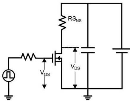
Figure 19. Dynamic R_DS(on) Test Circuit
