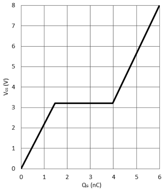
Figure 11. Typical Gate Charge
