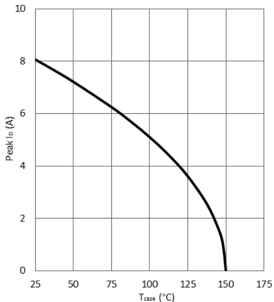
Figure 13. Current Derating
