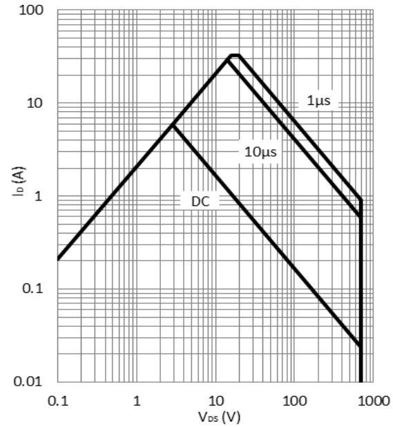
Figure 16. Safe Operating Area T C =80°C
