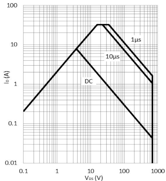
Figure 15. Safe Operating Area T C =25°C
