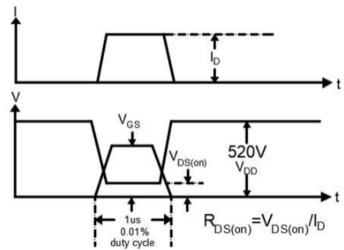
Figure 20. Dynamic R_DS(on) Waveform
