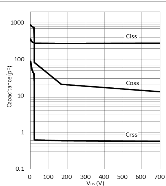
Figure 7. Typical Capacitance
