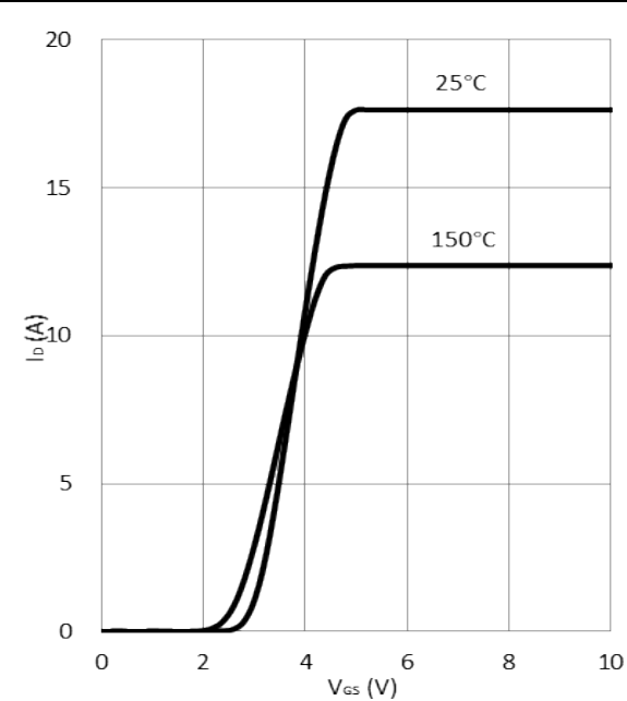
Figure 5. Typical Transfer Characteristics
