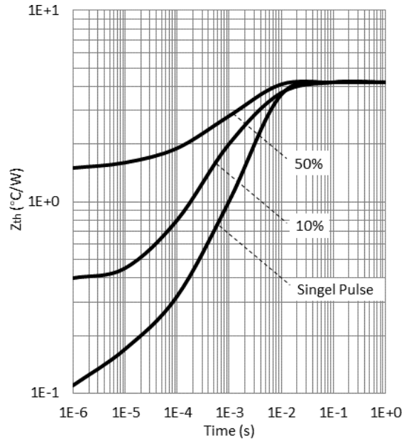
Figure 14. Transient Thermal Resistance
