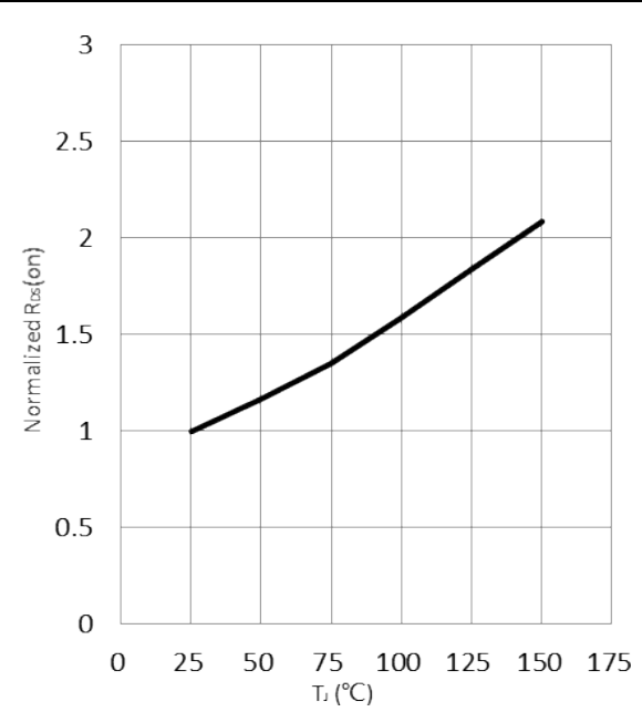
Figure 6. Normalized On-resistance
