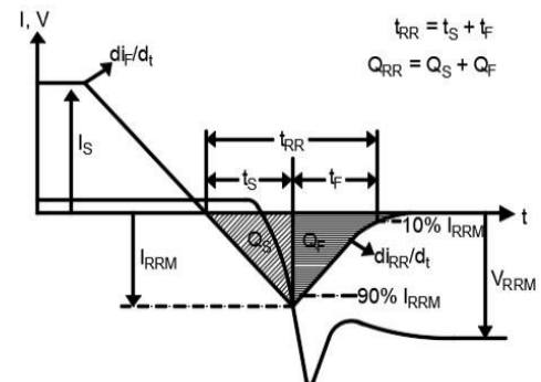
Figure 22. Diode Recovery Waveform
