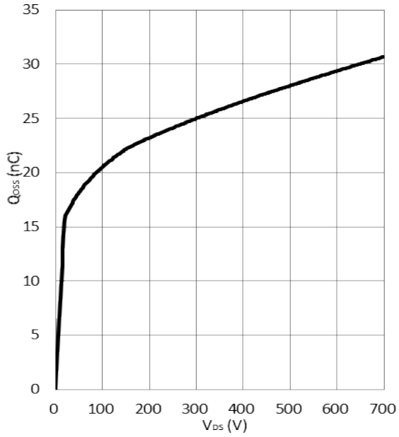
Figure 9. Typical Qoss
