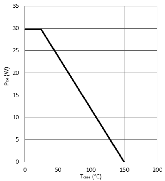
Figure 12. Power Dissipation
