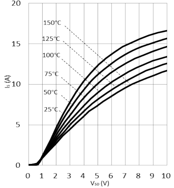
Figure 10. Forward Characteristic of Rev. Diode
